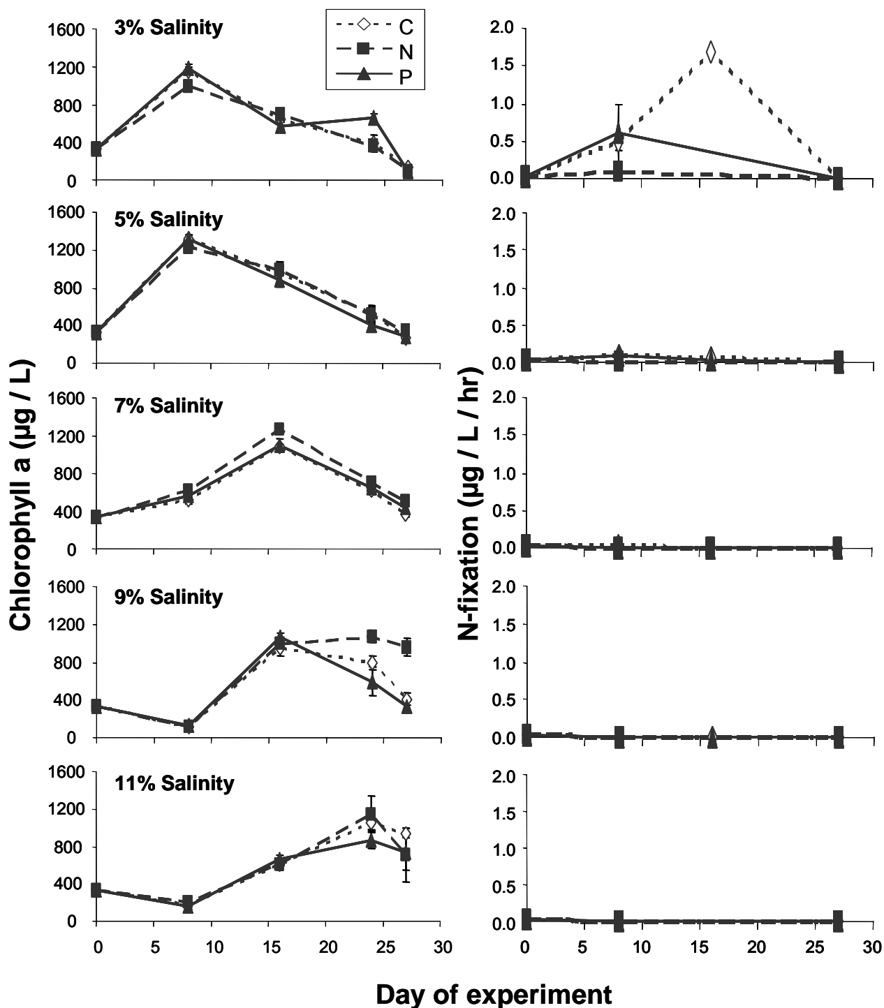
Figure 3: Responses of chlorophyll a concentrations (left) and nitrogen fixation (right) to nitrogen or phosphorus additions at five salinities with Farmington Bay water. Note the initial increase in chlorophyll in all treatments at low salinities, and delayed increases at higher salinities, with little difference between nutrient treatments except in the 9 and 11% salinities on days 24 and 28. Nitrogen fixation was only observed in the 3% treatment and was greatest in the control treatment. Day 24 nitrogen fixation data was omitted because sampling problems caused uncertainty in the results. Error bars \pm 1 S.E. C = Controls; N = +nitrogen; P = +phosphorus.
