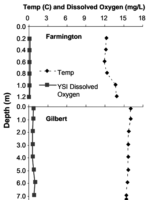
Figure 2: Temperature and oxygen profiles in Farmington and Gilbert Bays on 18 Oct 2004, when the water for the bioassays was collected. Note the different y-axis scales between the two panels. In Farmington Bay, there was inverse thermal stratification, indicating that the bay was underlain by a salt wedge. The entire water column was nearly anoxic. Oxygen concentrations were also low in Gilbert Bay, but there was no thermal or salinity stratification. Note that the hypersaline conditions in Gilbert Bay limit the amount of oxygen that can dissolve in the water. Oxygen and temperature were measured with a YSI Model 58 sensor, and the field concentrations were corrected for salinity and temperature.
